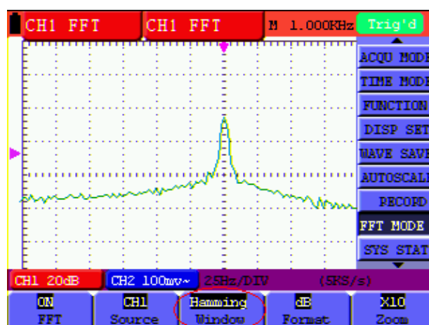
Fig.64. Hamming window
