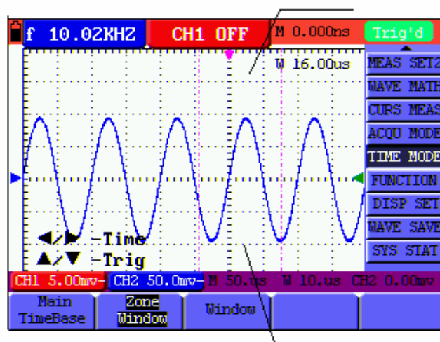
Figure 67: Window Setting
